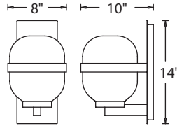
WS-W32714
